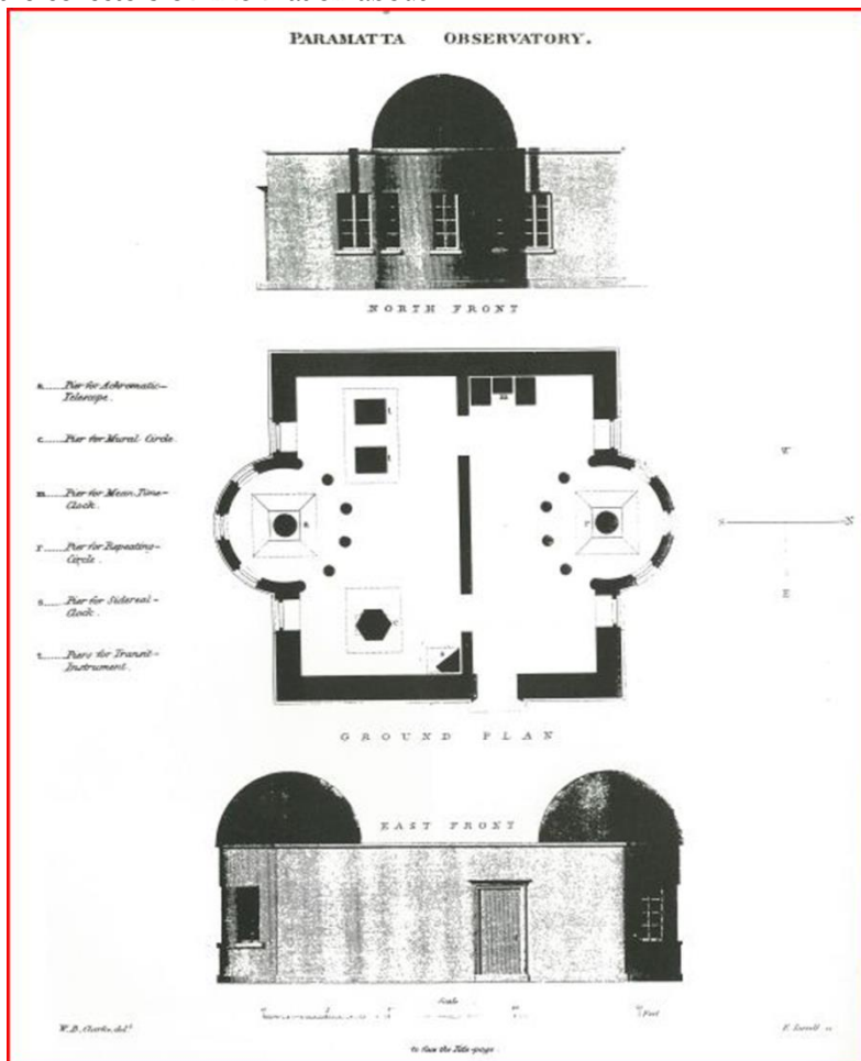
Figure 1. Plan of Parramatta Observatory drawn by Reverend W. B. Clarke. The locations of the Achromatic Telescope (a), Mural Circle (c), Mean-Time Clock (m), Repeating Circle (r), Sidereal Clock (s) and Transit Instrument (t) are shown in the figure.
